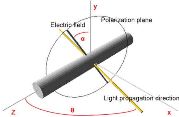
Fig. 1 - Geometry used in our three dimensional model.
