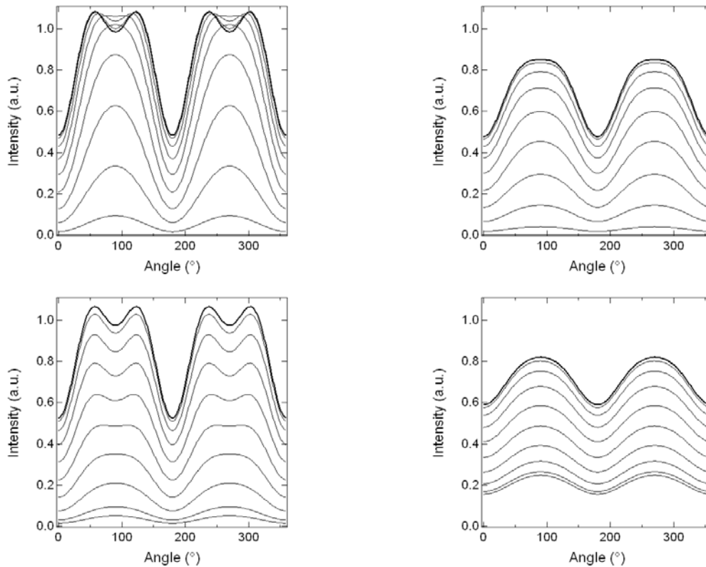
Fig. 2 - Evolution of the polarization profiles in model 1 (top) and model 2 (bottom) for different values of \theta (from 90^\circ to 0^\circ within each panel) and \sigma ( 10^\circ , left and 30^\circ , right).
