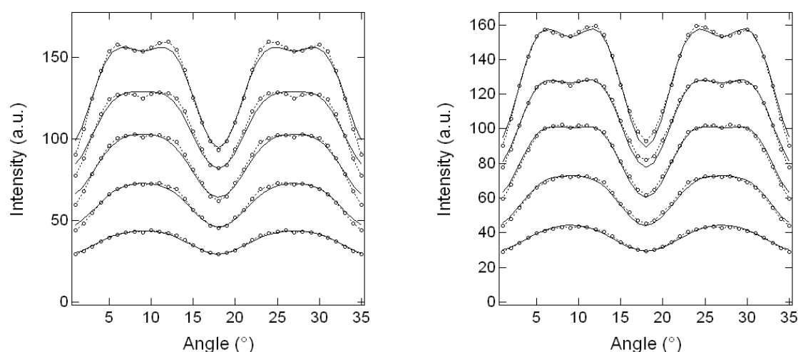
Fig. 3 - Experimental data fitted with the completely coherent (left) and with the completely incoherent (right) model.
