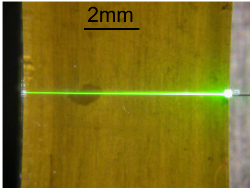
Channel waveguide
